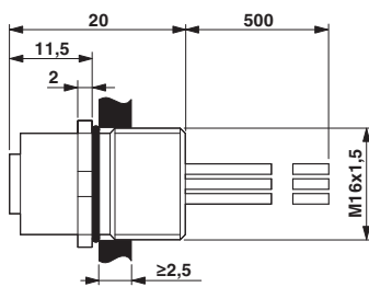
Dimensional drawing
